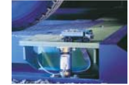
C16-load corner, the worldwide leading solution for truck scales
